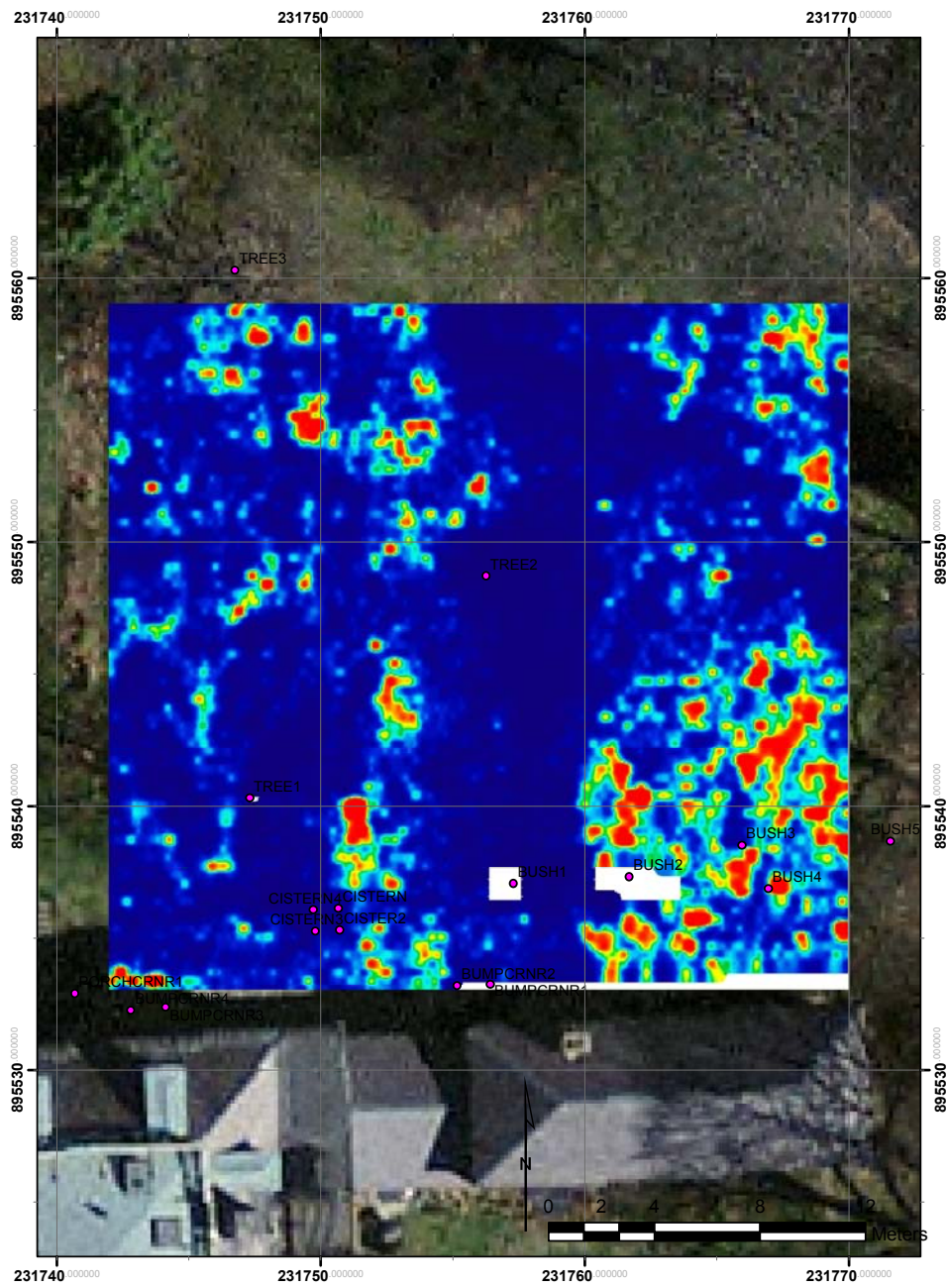
Figure 25. GPR slice of 170-180 cm bgs.
