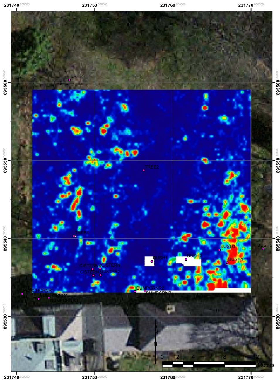
Figure 28. GPR slice of 200-210 cm bgs
