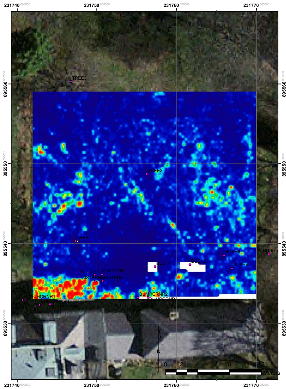
Figure 16. GPR slice of 80-90 cm bgs. Hard reflectors are in red.
