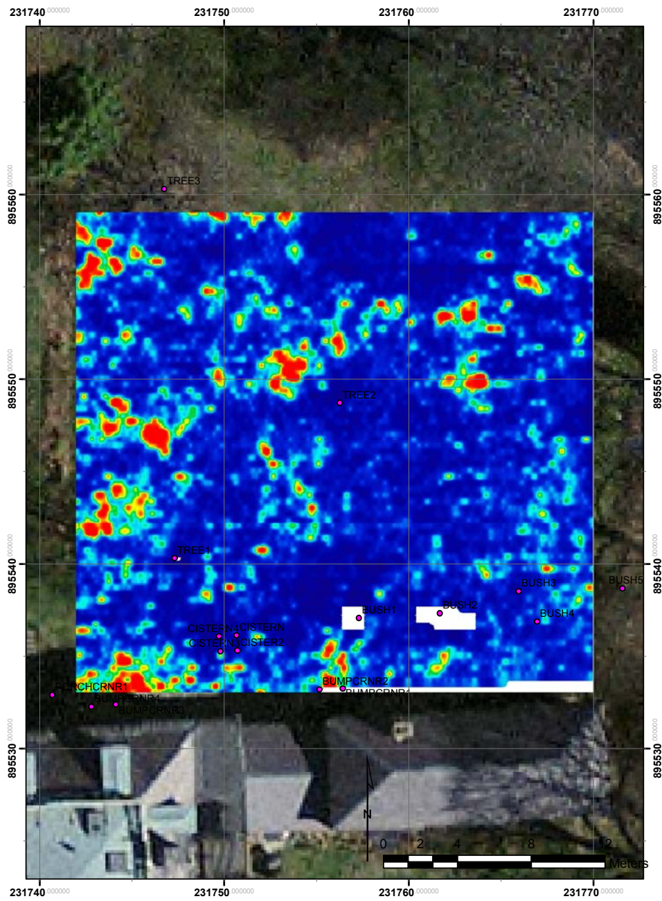
Figure 36. GPR slice of 280-290 cm bgs
