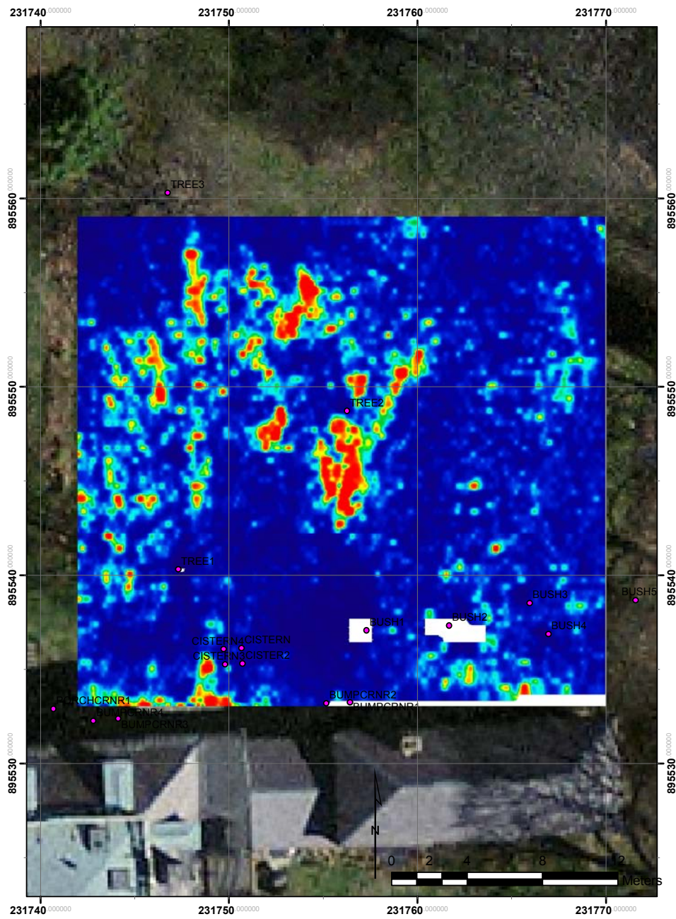
Figure 18. GPR slice of 100-110 cm bgs. Hard reflectors are in red.
