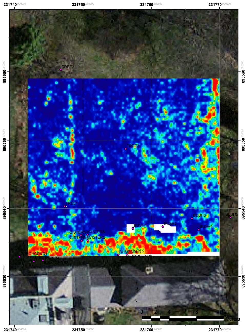
Figure 14. GPR slice of 60-70 cm bgs. Hard reflectors are in red.
