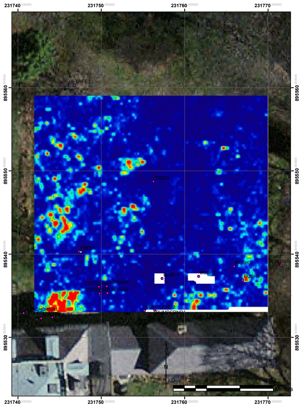
Figure 32. GPR slice of 240-250 cm bgs
