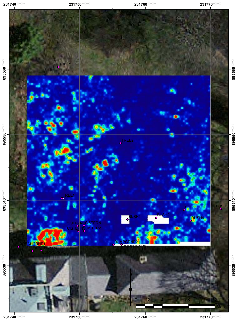
Figure 31. GPR slice of 230-240 cm bgs
