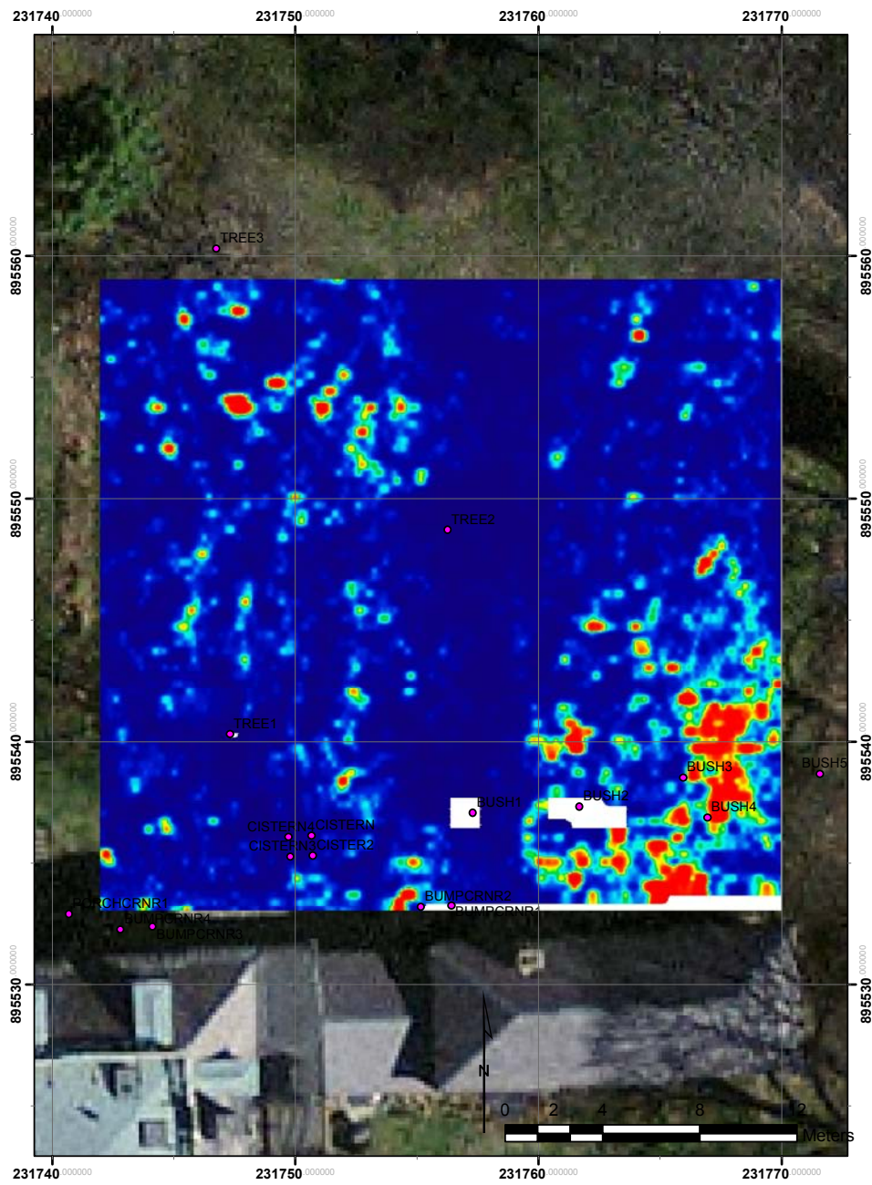
Figure 27. GPR slice of 190-200 cm bgs
