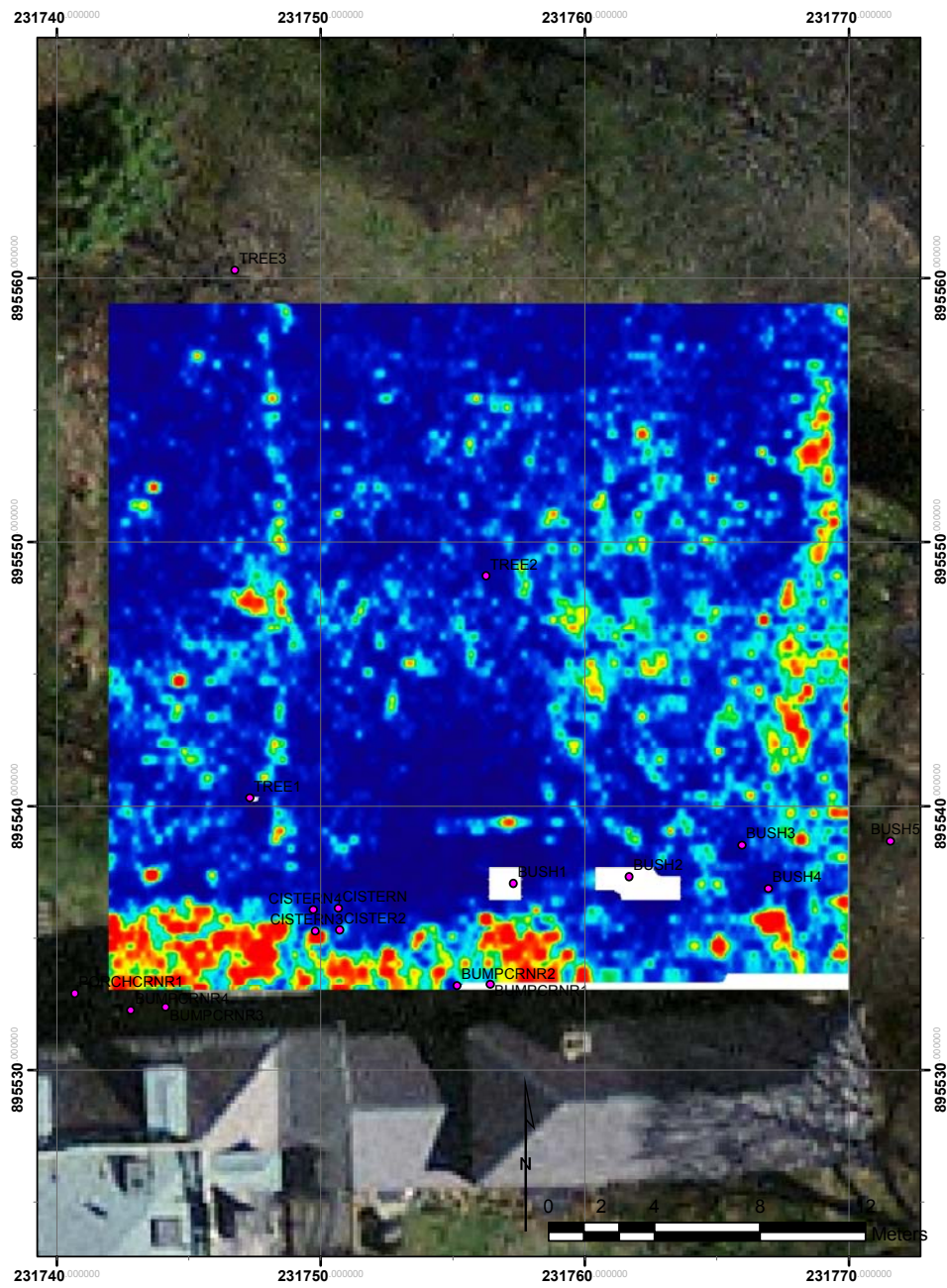
Figure 15. GPR slice of 70-80 cm bgs. Hard reflectors are in red.
