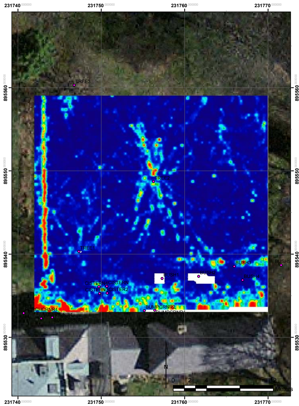
Figure 11. GPR slice of 30-40 cm bgs. Hard reflectors are in red.
