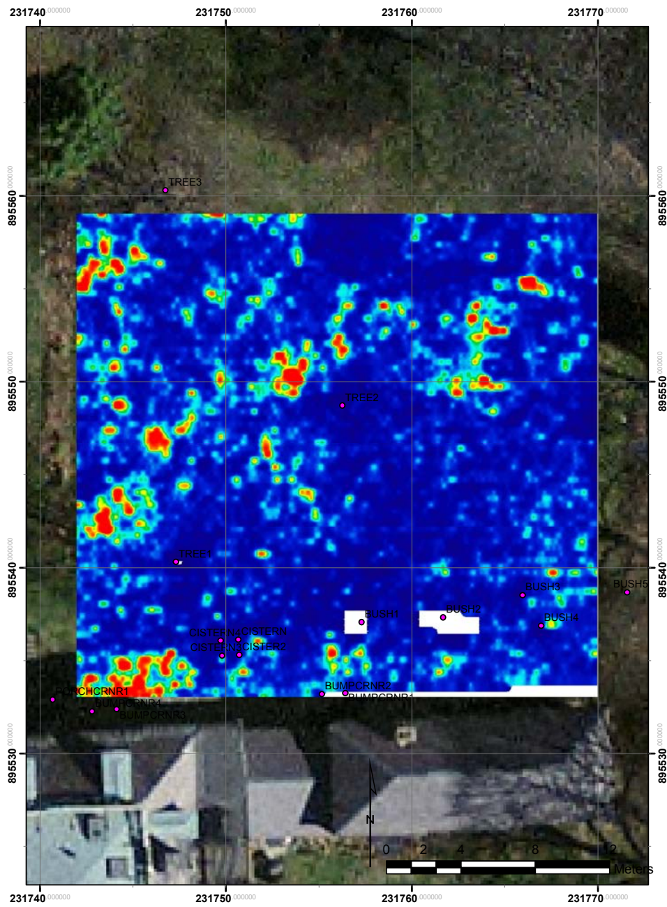
Figure 35. GPR slice of 270-280 cm bgs
