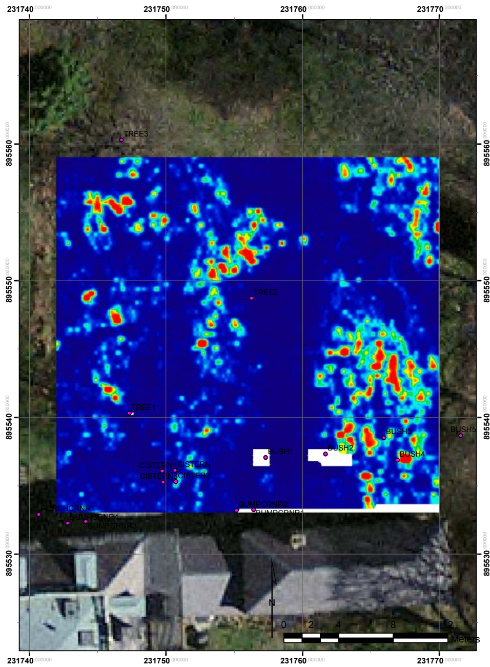
Figure 23. GPR slice of 150-160 cm bgs.
