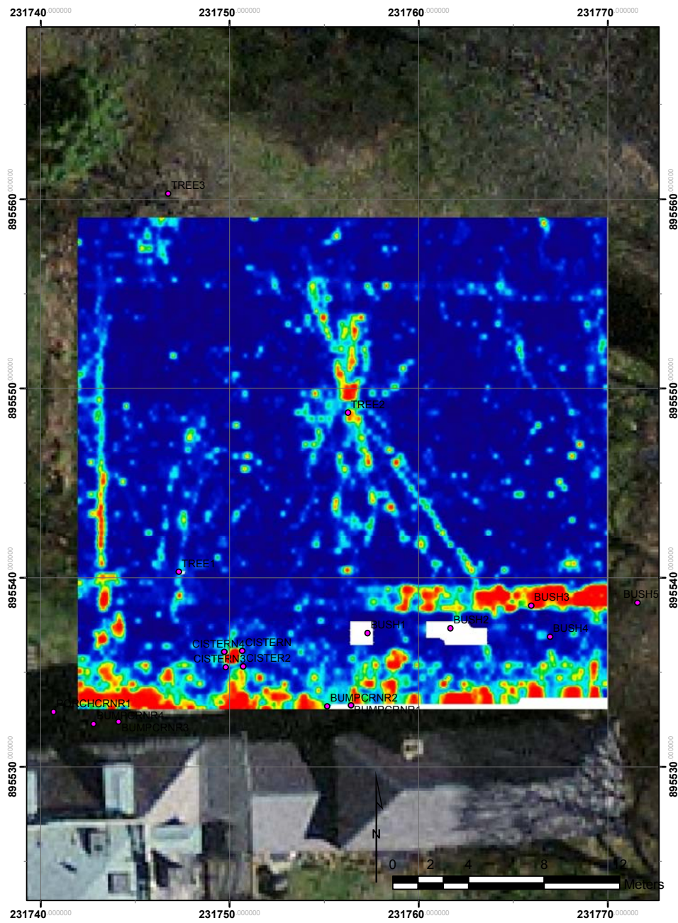
Figure 10. GPR slice of 20-30 cm bgs. Hard reflectors are in red.
