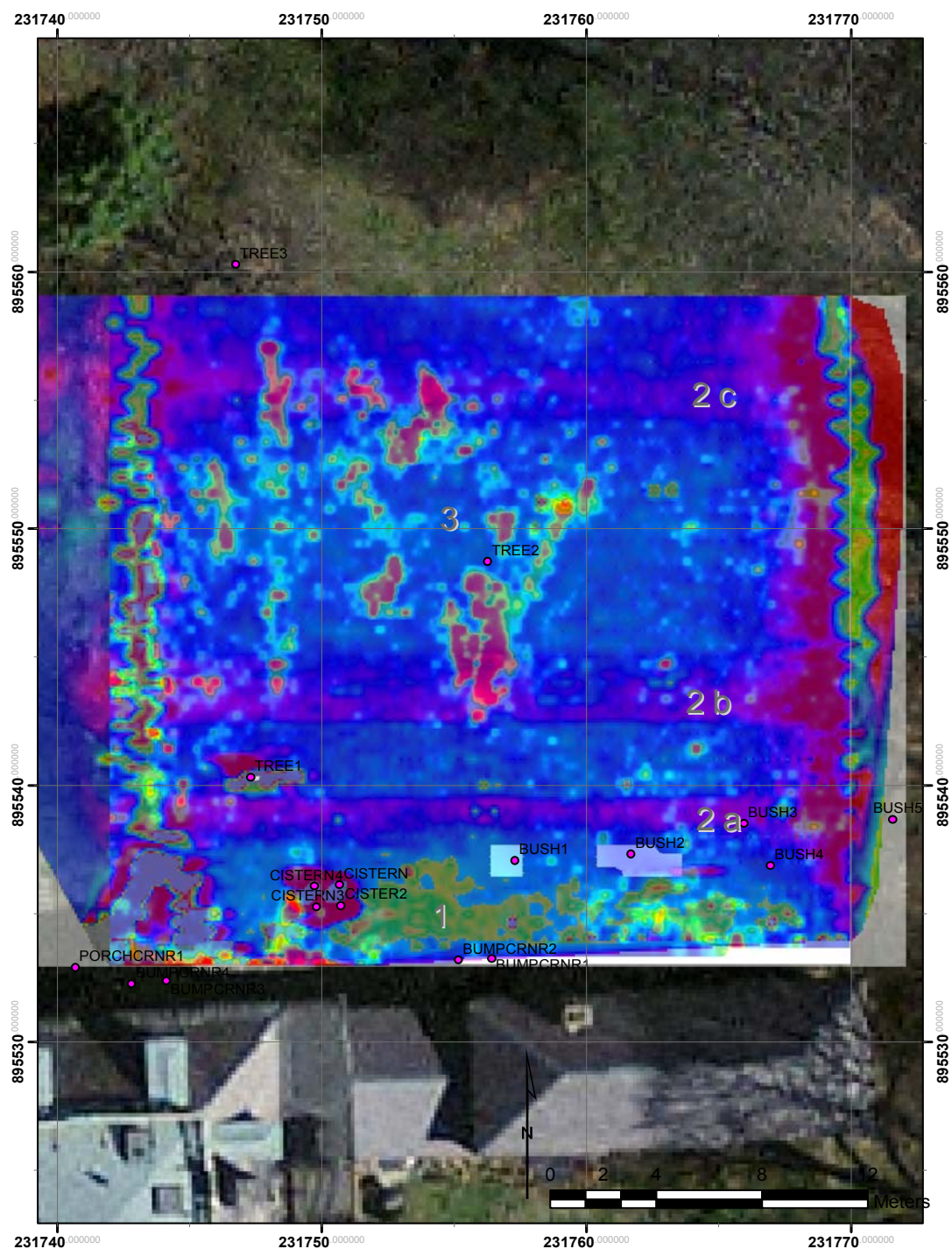
Figure 43. Anomaly 1 (builders trench), Anomaly 2 (garden paths), and Anomaly 3 (possible house foundation) are labeled on the air photo. Underneath the labels is the EM-38 map as well as the 110-120 cm bgs GPR slice.
