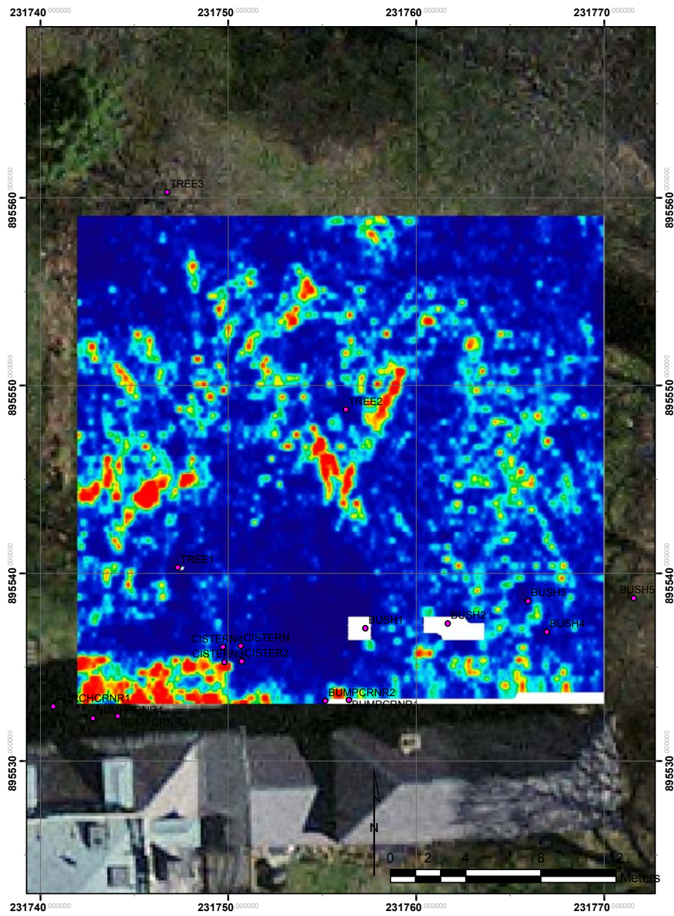
Figure 17. GPR slice of 90-100 cm bgs. Hard reflectors are in red.
