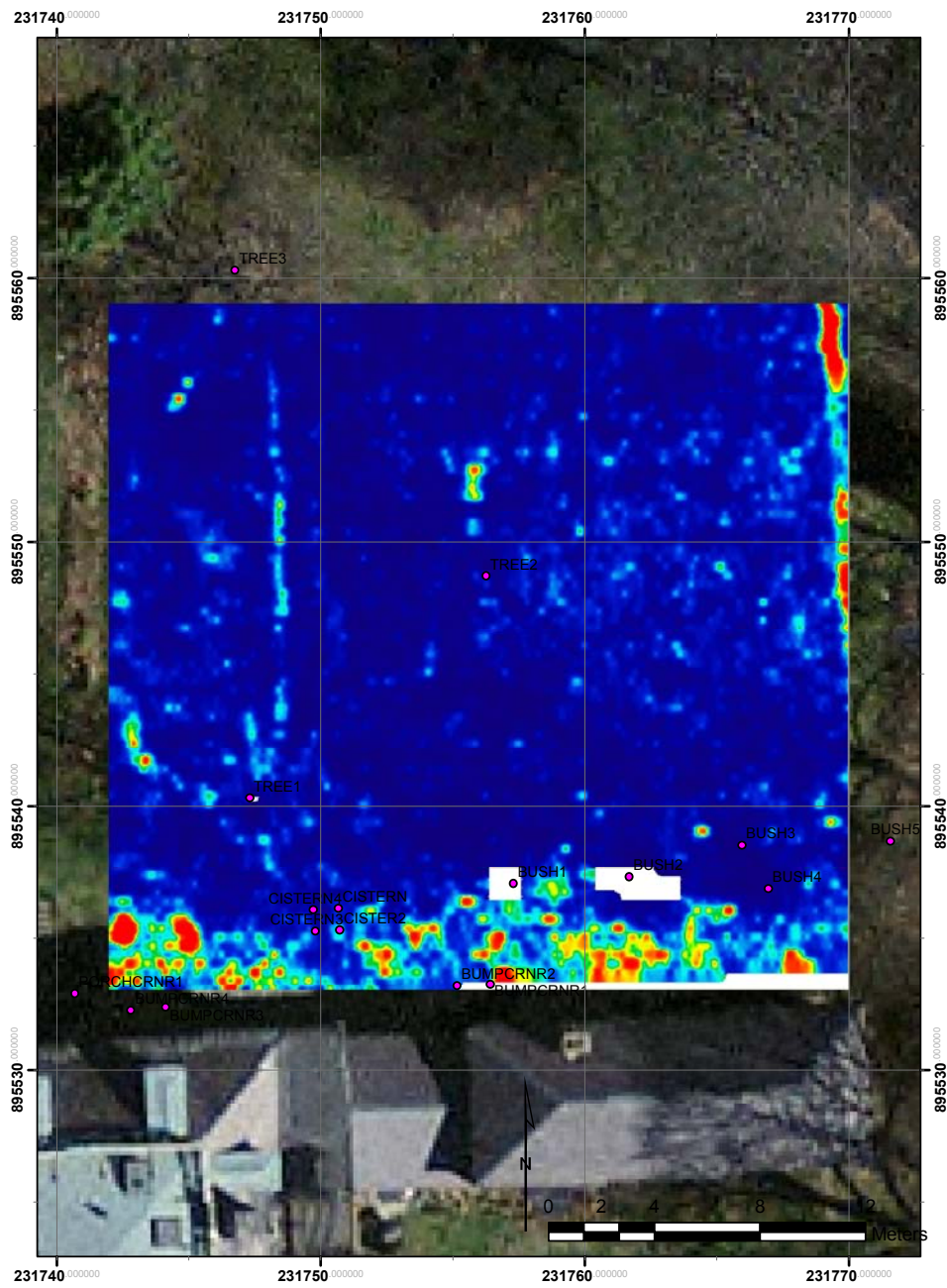
Figure 13. GPR slice of 50-60 cm bgs. Hard reflectors are in red.
