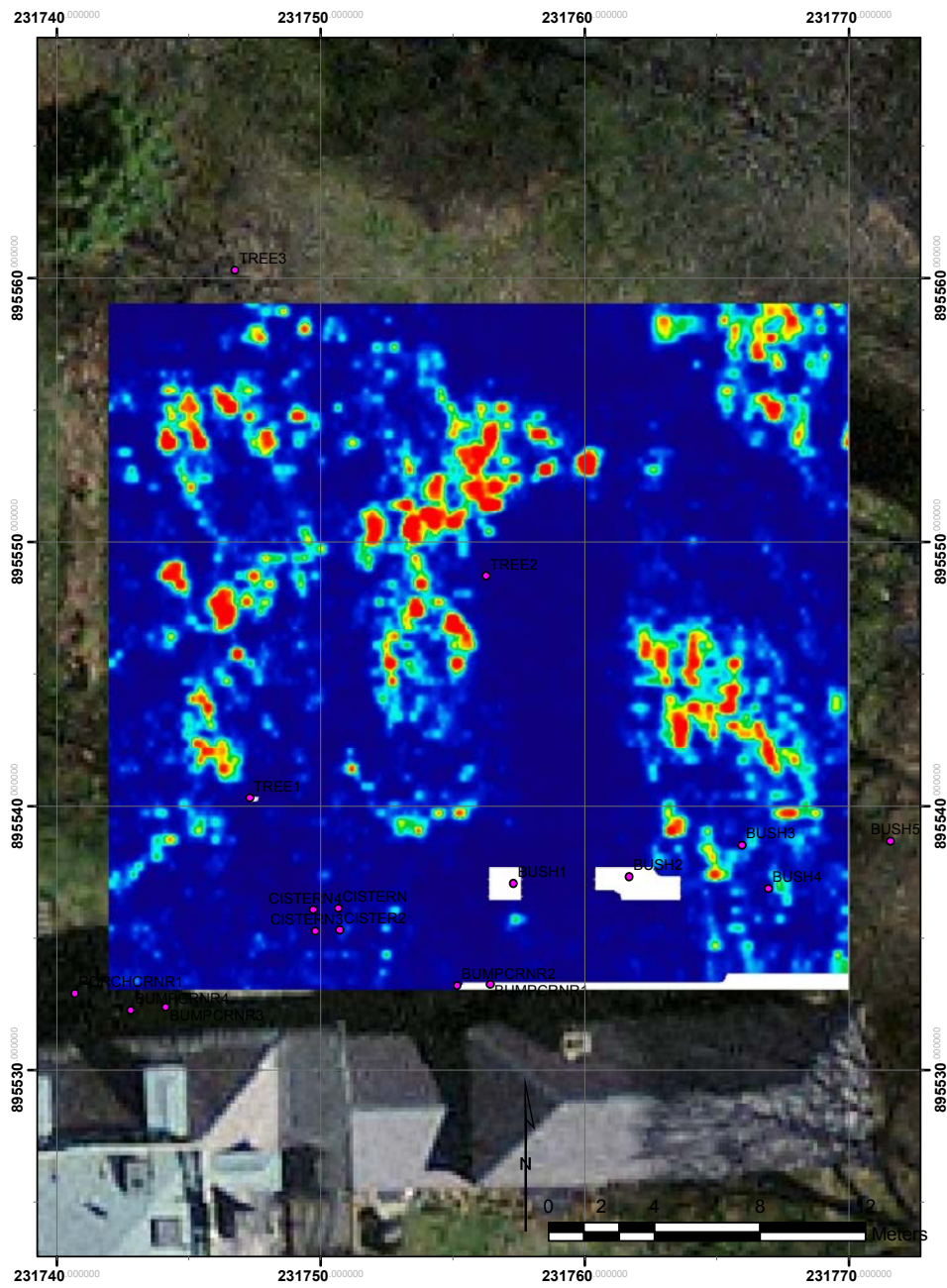
Figure 22. GPR slice of 140-150 cm bgs.
