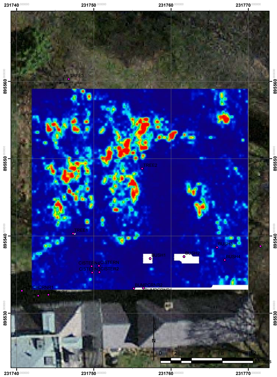
Figure 21. GPR slice of 130-140 cm bgs
