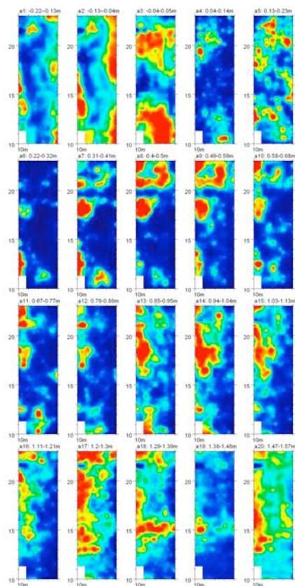
Figure 38. GPR slices from 500 MHz antenna of strip of backyard at 428 Thames, Newport RI. The well is centered on E 11 , N 18 . The well signature starts to appear in the 4-14 cm bgs slice (a 4 ) and continues strongly through 120-130 cm bgs (a 17 ).
