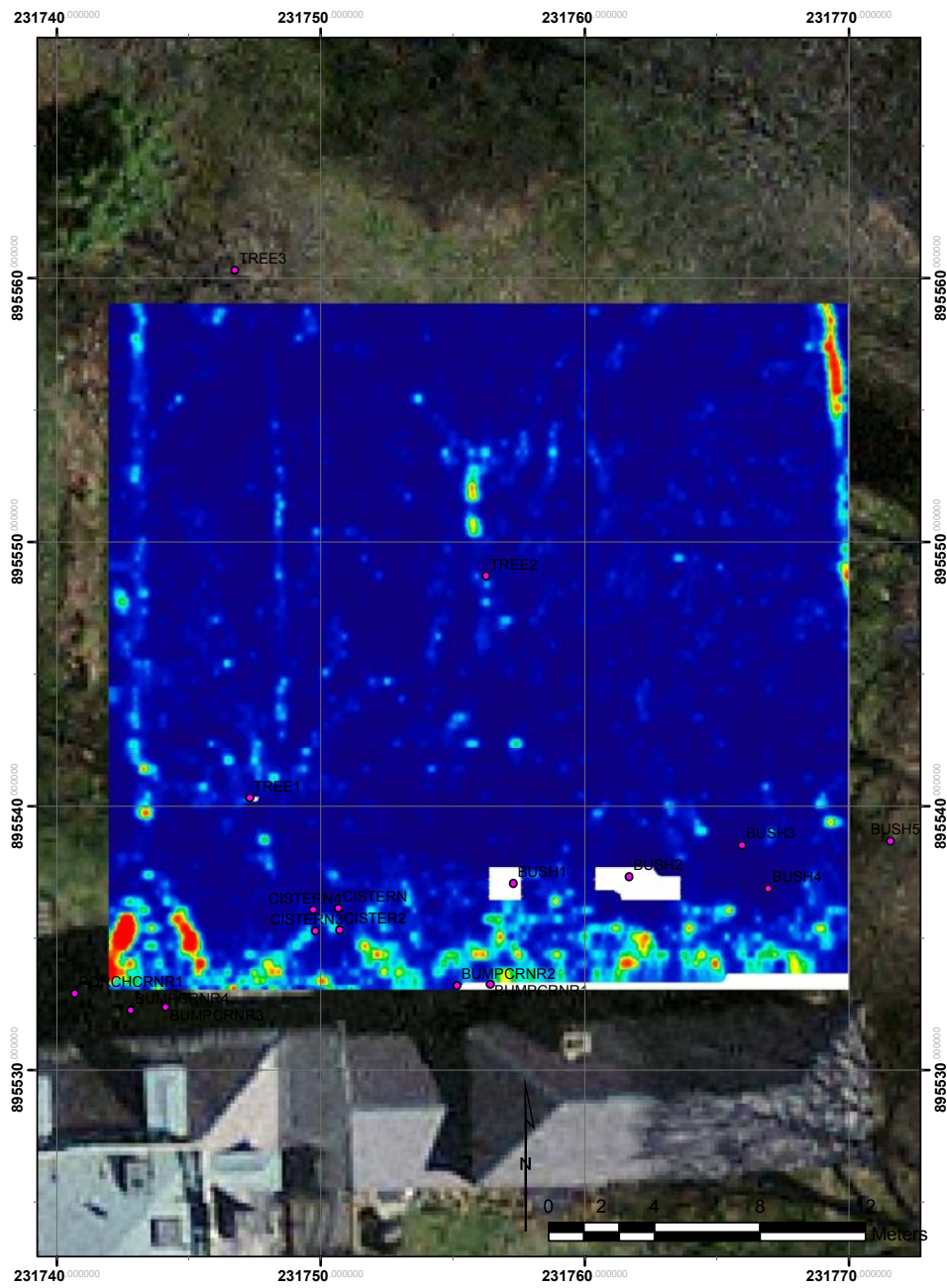
Figure 12. GPR slice of 40-50 cm bgs. Hard reflectors are in red.
