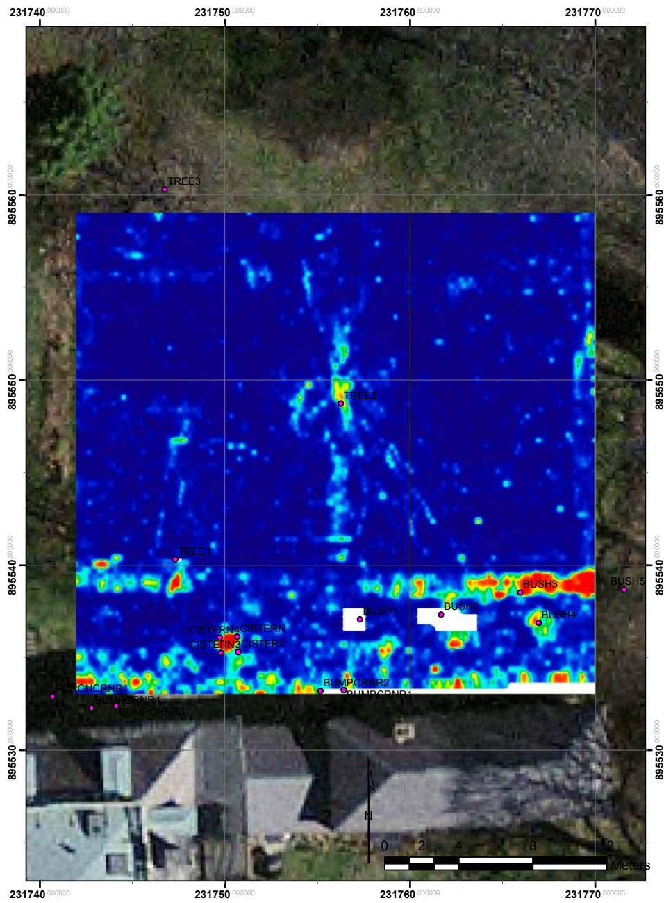
Figure 9. GPR slice of 10-20 cm bgs. Hard reflectors are in red.
