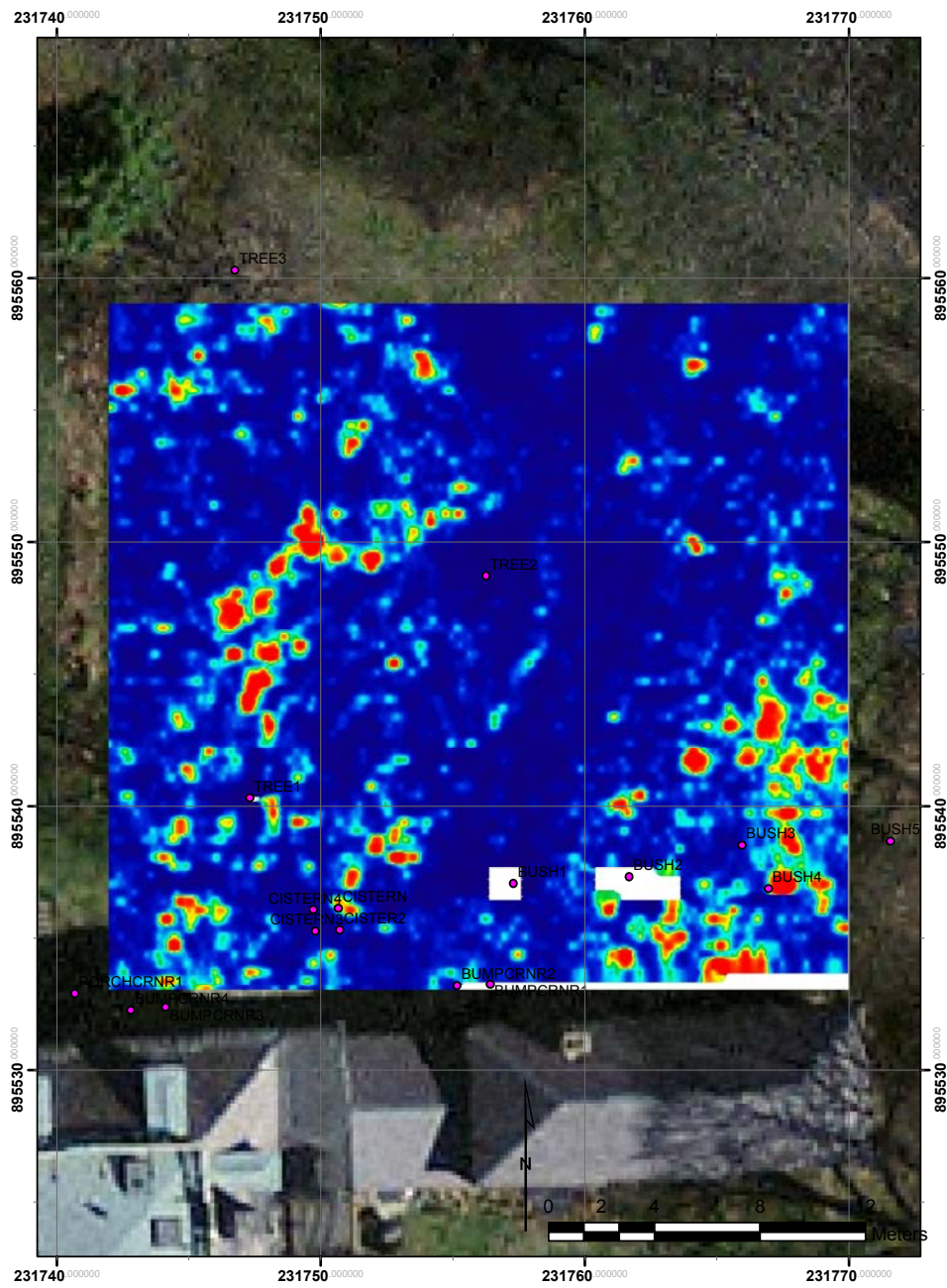
Figure 29. GPR slice of 210-220 cm bgs
